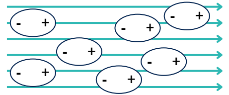
Arrangement of non-polar molecules under the influence of a magnetic field
