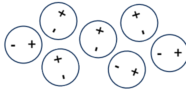
Arrangement of non-polar molecules in the absence of a magnetic field
